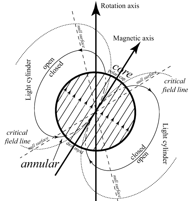
Fig. 1 A schematic illustration of an isolated (i.e., without accretion) quark star and its magnetospheric geometry. The quark star is suggested to be homogeneously magnetized due to the speculation of magnetic symmetry broken spontaneously in solid quark matter as the star cools to a temperature to be lower than a critical Curie temperature.
