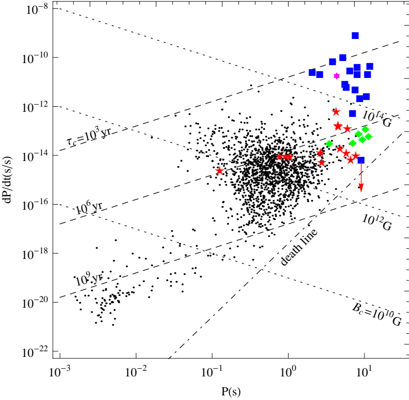
Fig. 1. P-\dot{P} diagram of pulsars. Squares are for AXP and SGRs, the six-pointed-star is for the radio loud magnetar, the down-arrow marks the low magnetic field SGR (from McGill online catalog: http://www.physics.mcgill.ca/~pulsar/magnetar/main.html ). Diamonds are for X-ray dim isolated neutron stars (XDINSs) (from Kaplan & van Kerkwijk 2011). Stars are for rotating radio transients (RRATs), dots are for normal and millisecond pulsars (from ATNF: http://www.atnf.csiro.au/research/pulsar/psrcat/ ).
