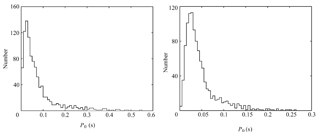
Fig. 1 Histograms for the initial period P_0 . Left: P_0 is calculated from B_{12} = 0.0637P_0^{-1} , in which data of 997 pulsars are used and each bin represents an interval of 10 ms. Right: P_0 is calculated from B_{12} = 8.24 \times 10^{-1.5}P_0^{-1.5} , in which data of 1046 pulsars are plotted and each bin represents 5 ms.
